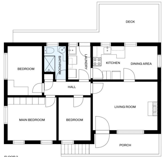
FLOOR 2
